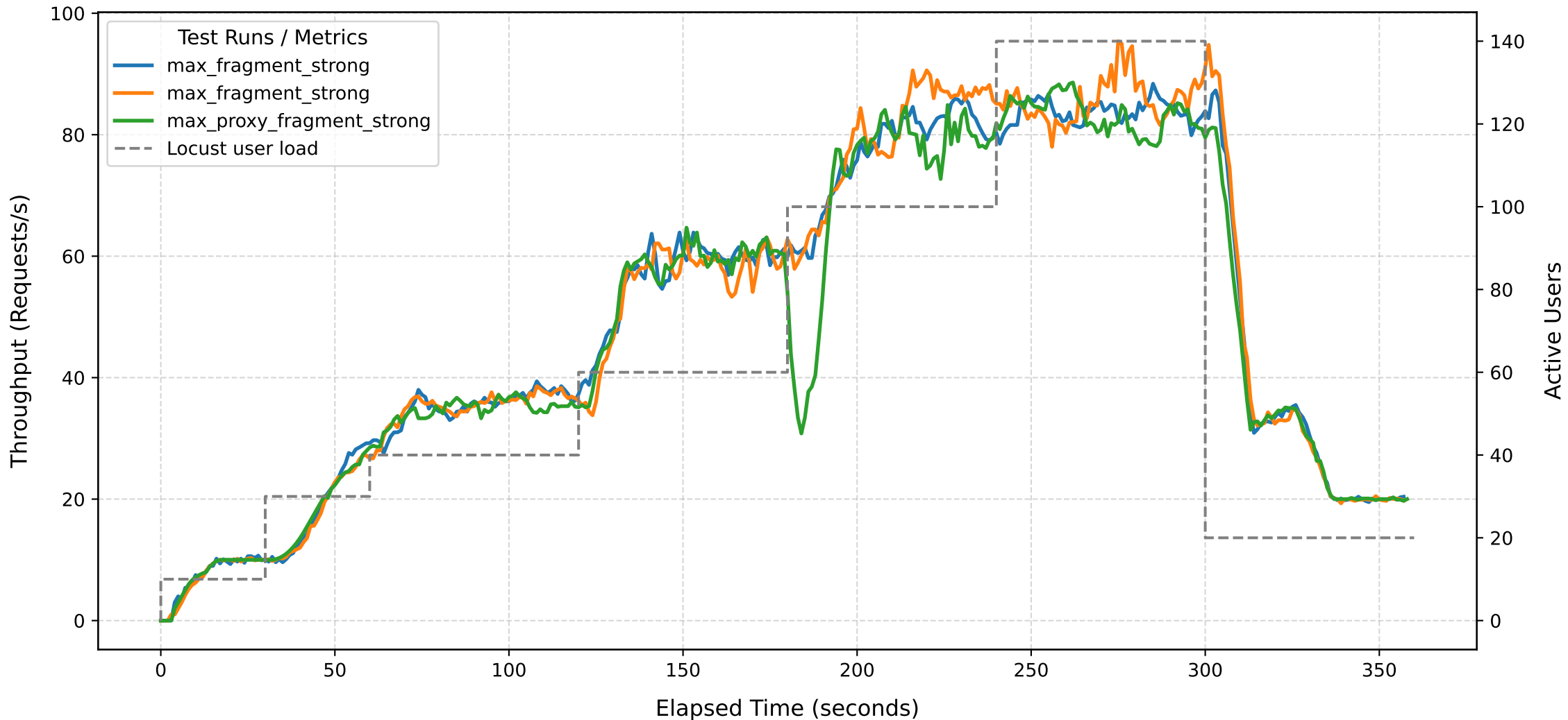
Locust Performance Test - Throughput (RPS) Comparison
